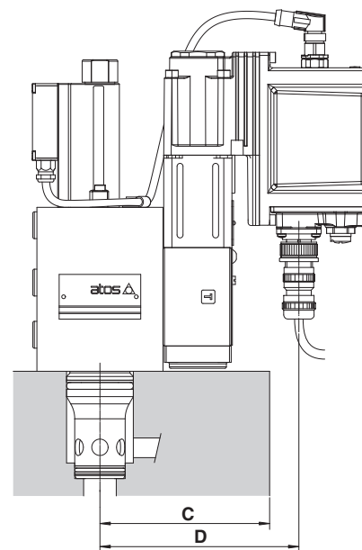
Installation 2 - no interference
