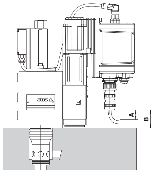
Installation 1 - possible interference between manifold and main connector
