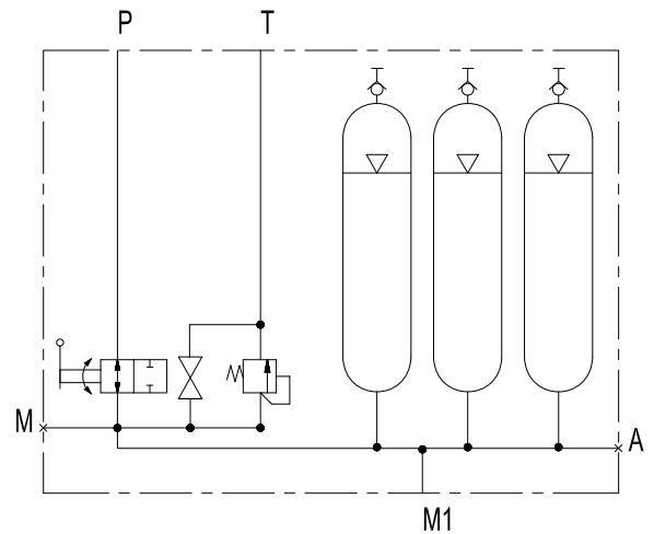
HYDRAULIC DIAGRAM
