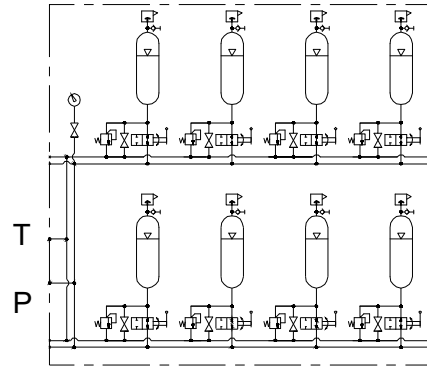
HYDRAULIC DIAGRAM
