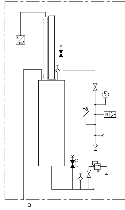
HYDRAULIC DIAGRAM
