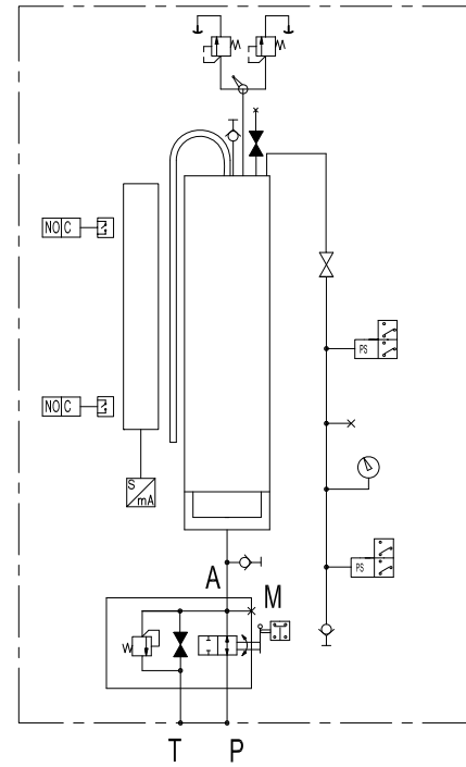
HYDRAULIC DIAGRAM
