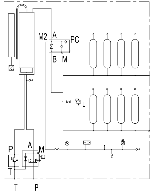
HYDRAULIC DIAGRAM
