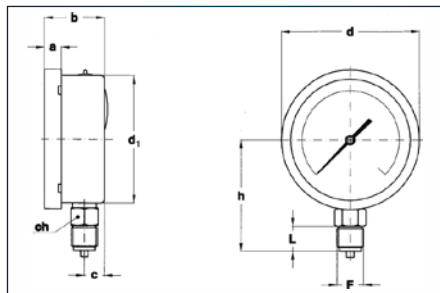
A Manometry radialne / Lower connection
